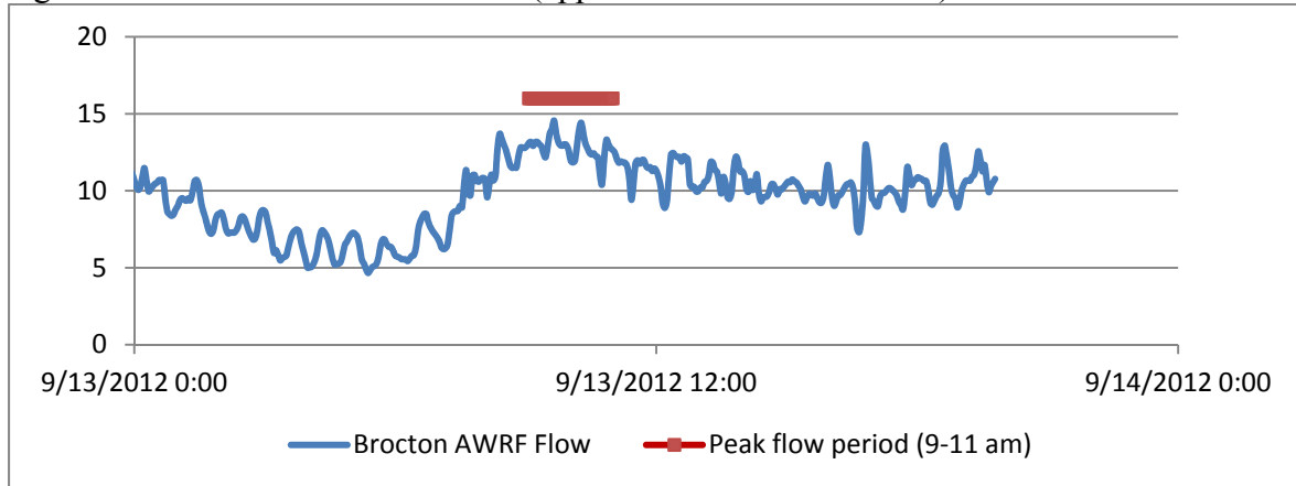
Figure B-3. Brockton AWRP Flows (approx. 3-min SCADA data)
